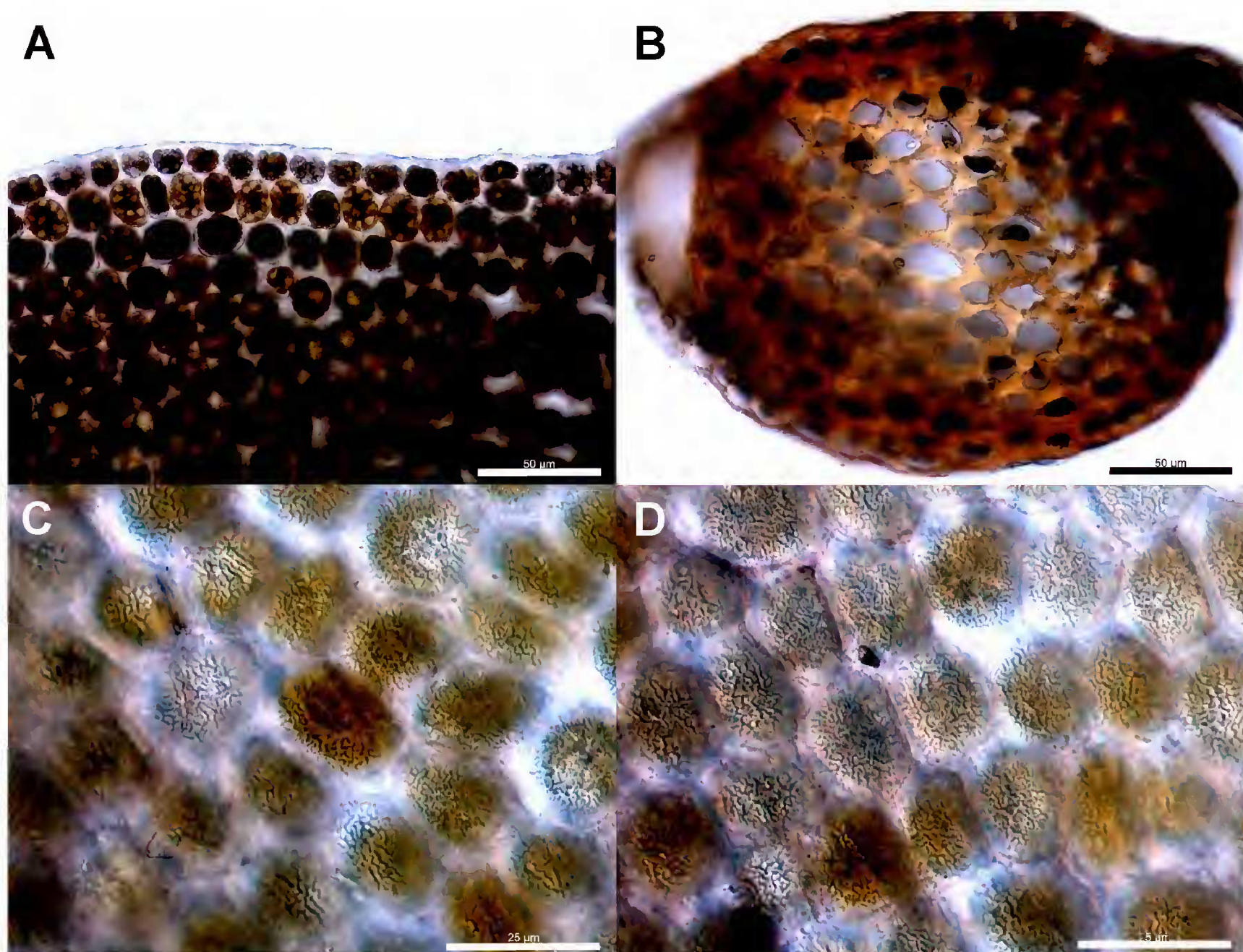
Fig. 6. Radula oreopsis Plate B. A: Leaf-lobe margin (50 \mu\text{m} ). B: Transverse section of primary stem (50 \mu\text{m} ). C, D. Leaf-lobe medial cell surface, showing ruminant ornamentation (25 \mu\text{m} ). All from NSW896698.
